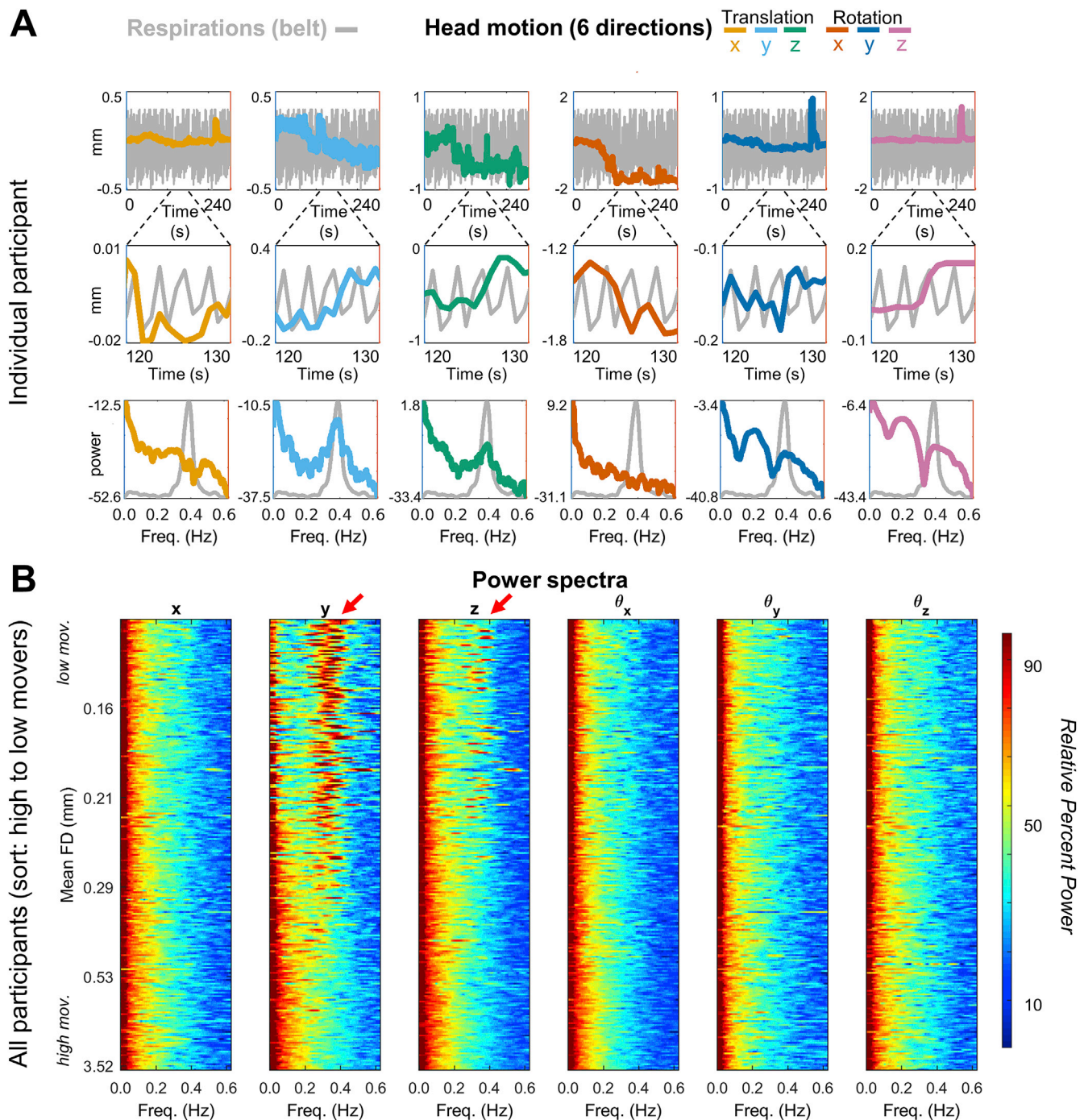
Fig. 5. Frequency domain representation of motion time series in multiband data. (A) One fMRI run in a single representative ABCD participant ( TR = 800 ms). Colored lines represent the translation and rotation motion estimates. Top row: entire (240 s) fMRI run; middle-row: 10 s ‘snapshot’; Bottom row: power spectra of the motion and respiratory belt traces. (B) Power spectra of 62 OHSU ABCD-study participants (mean age 11.6, TR = 0.8 s), ordered by mean FD and stacked with lowest movers on top. Red arrows highlight characteristic frequency of respiration artifact ( \sim 0.3 Hz). To allow for visual comparisons across a wide range of motion time series power, (i.e., with and without filtering – Fig. 5 and 6 and SI Fig. 2 and 3) the spectra were first represented logarithmically (i.e., in dB) and then Z-scored (details in Appendix B); replication of these figures in one’s own data can be conducted with code provided by github.com/DCAN-Labs . Thus, the respiratory peak is suppressed in very high motion data, which are dominated by low frequency power.
