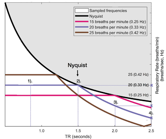
Fig. 7. Respiratory artifact aliasing as a function of sampling rate. (A) BOLD data were collected while the participant's respiratory rate was visually paced at exactly 0.33 Hz (20 breaths/min; see Supplementary Movie 1) at TRs of 1). 0.8 s (multiband), 2). 1.5 s (multiband), 3). 2.0 s (multiband) and 4.) 2.5 s (singleband). The respiratory belt data were sampled at the same rate as the BOLD data for each TR (e.g. for a TR of 2.0 s, respiration data (gray) were sampled every 2.0 s). Note that the peak power for the respiration (gray) and head motion traces (6 directions) overlap closely and are moved to lower frequencies by sampling at larger intervals (1–4). (B) Superimposition of empirical spectral peak values over predicted values based on Nyquist theory as outlined in Methods. For sampling rates of 1). 0.8 s and 2). 1.5 s there is no aliasing and the respiratory peak stays at 0.3 Hz. For sampling rates of 3). 2.0 s and 4). 2.5 s the respiratory peak gets aliased to lower frequencies (marked by purple 'X'). Note close match of empirical (A) vs. theoretical (B) spectral peak frequencies.
